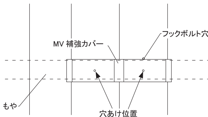
MV 補強カバーの仮置
